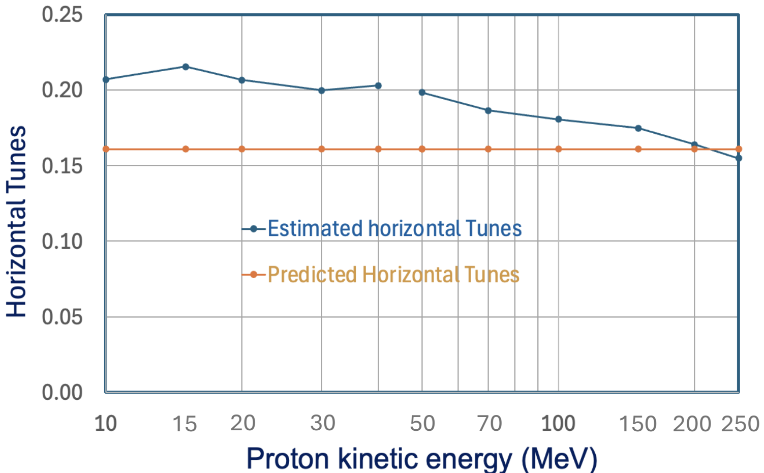
Initial Horizontal tune vs. energy analysis
