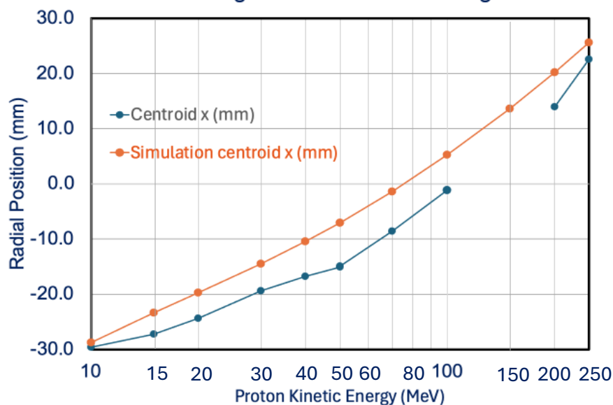
Beam Out Flag Centroid Positions Flag #3
