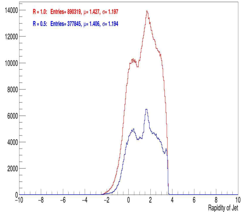
Jet Rapidity Distribution
