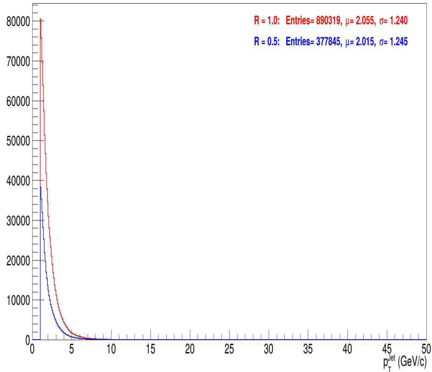
Jet Momentum
