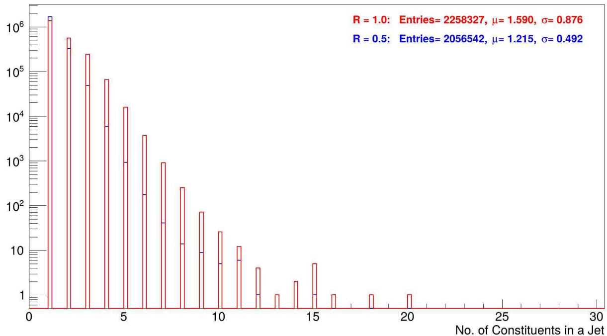
Jet Constituents
