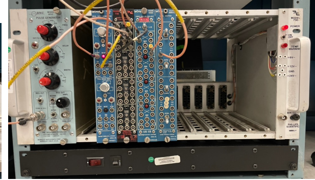
NIM crate with fast logic
