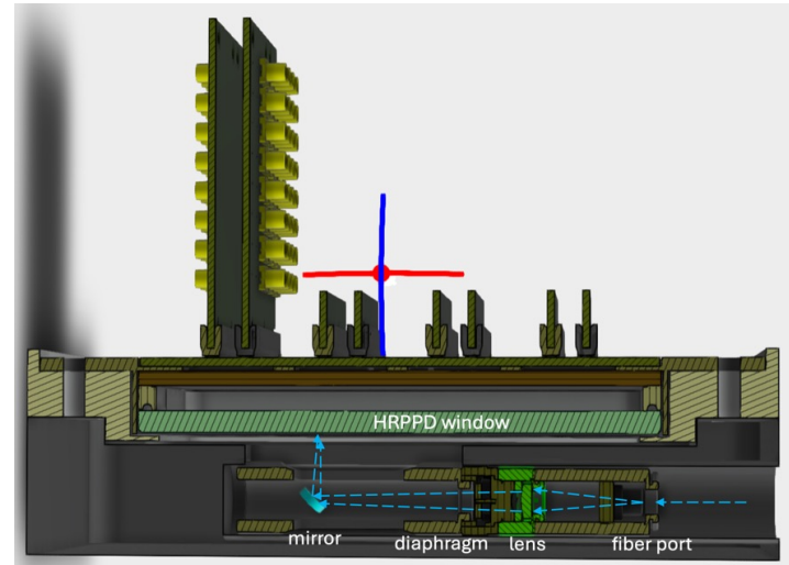
HRPPD enclosure; can be tilted in 2D; fiber-coupled to the PiLas laser
