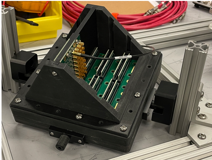
HRPPD enclosure; can be tilted in 2D; fiber-coupled to the PiLas laser
