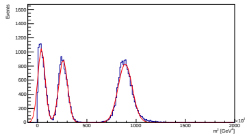
1.5 \leq p < 2.0 m^2 spectrum [MeV ^2 ]
