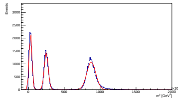
1.0 \leq p < 1.5 m^2 spectrum [MeV ^2 ]
