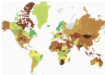
Electricity-related emissions by region [1].
