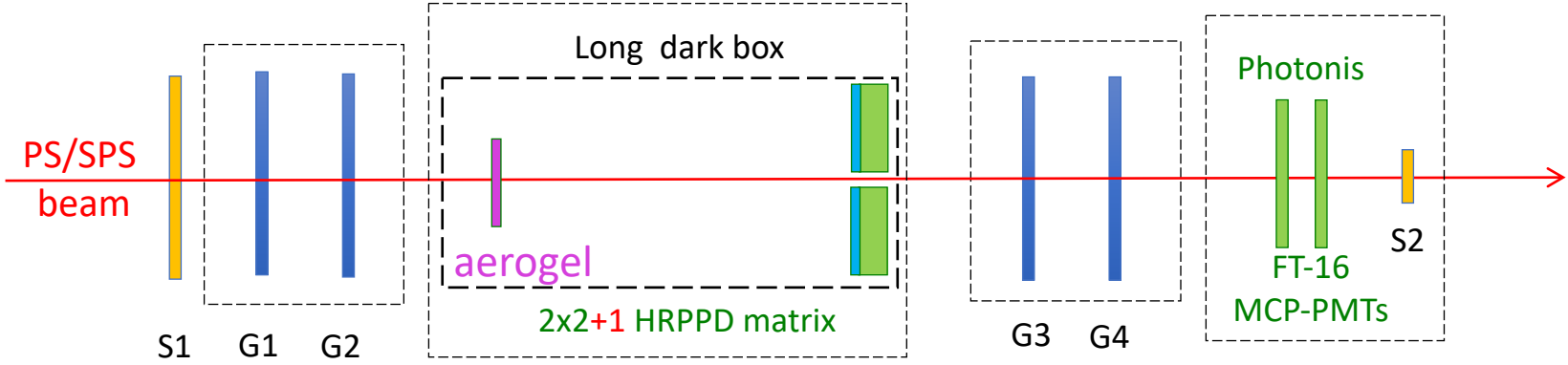
S1&S2: trigger scintillators; G1..G4: GEM trackers
