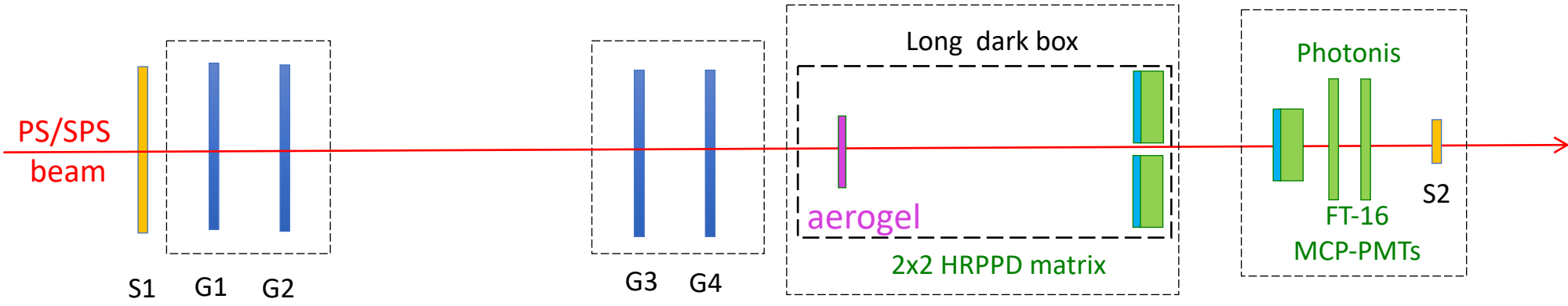
S1&S2: trigger scintillators; G1..G4: GEM trackers
