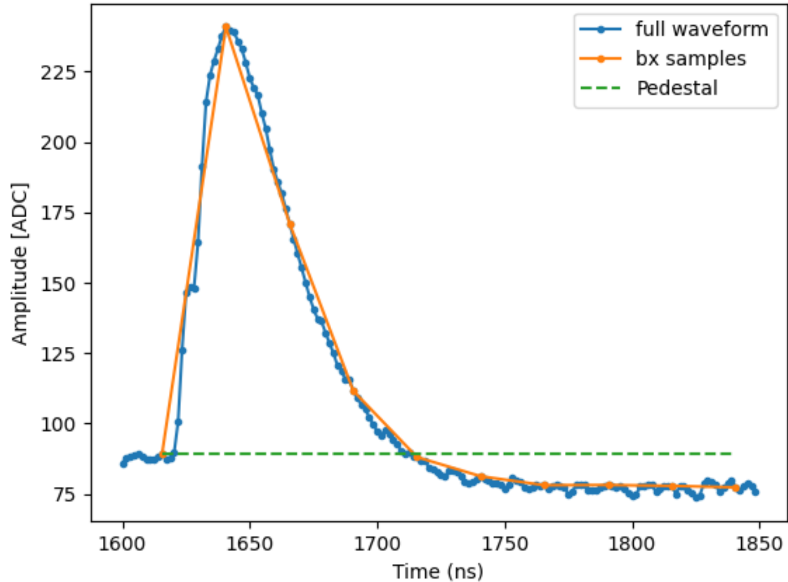
Signal vs time for channel 35 with a phase offset of 11
