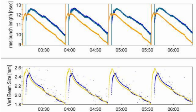
Operational 3D cooling of Au ions during RHIC Run 2020.
