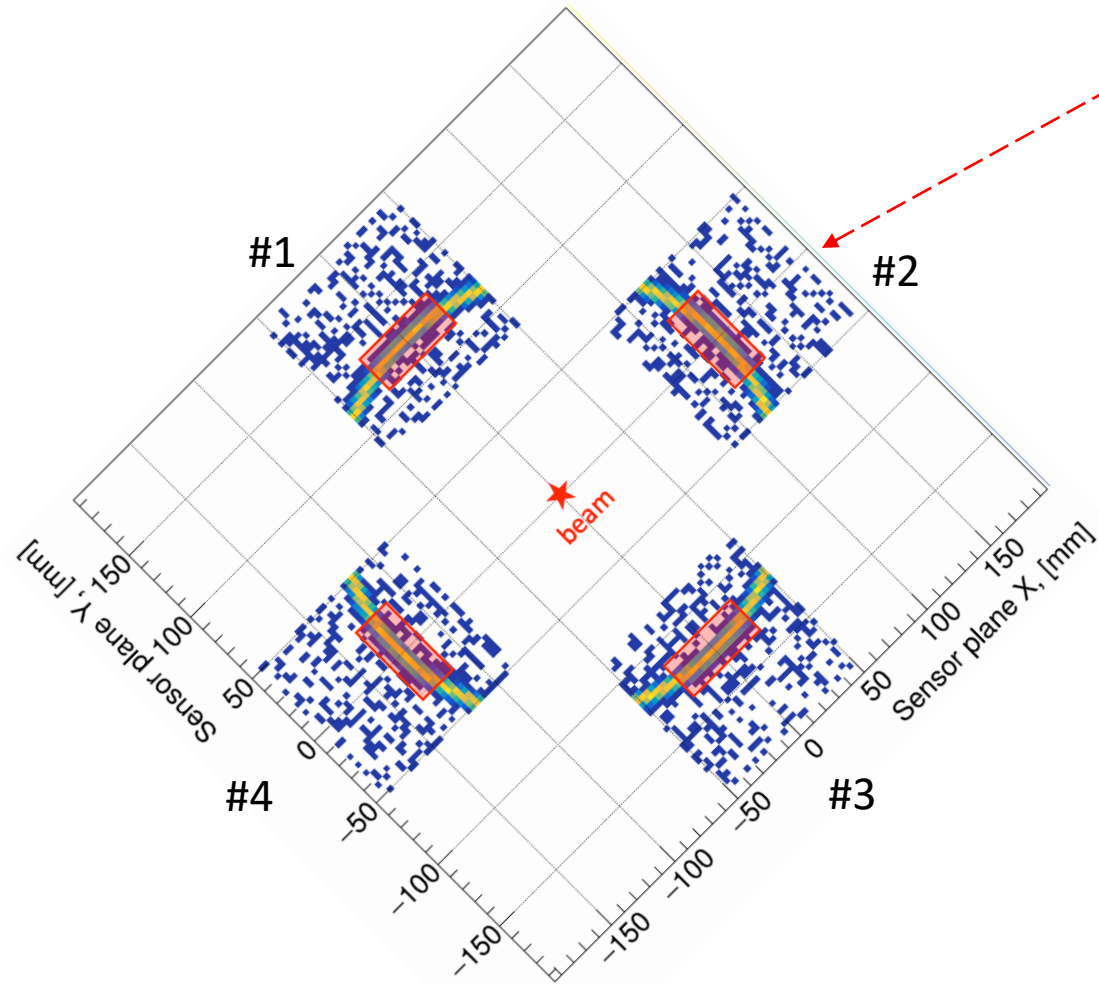
Instrumented 2x2 HRPPD area
