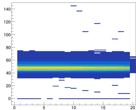
Waveform channel 122
