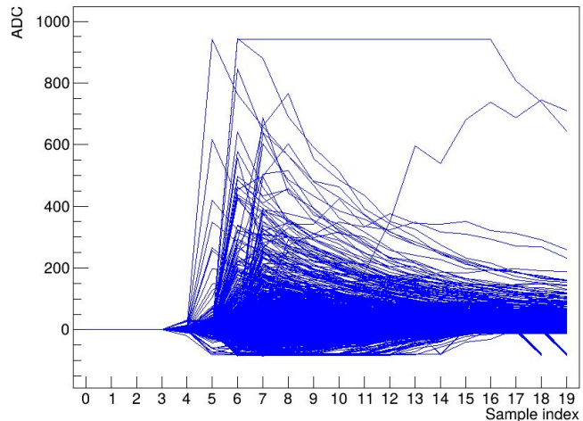
Baseline corrected | Ch 33
