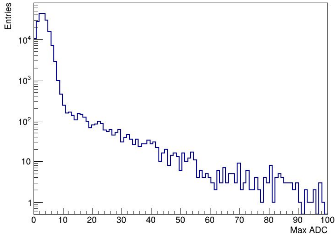
Max ADC distribution | Channel 33
