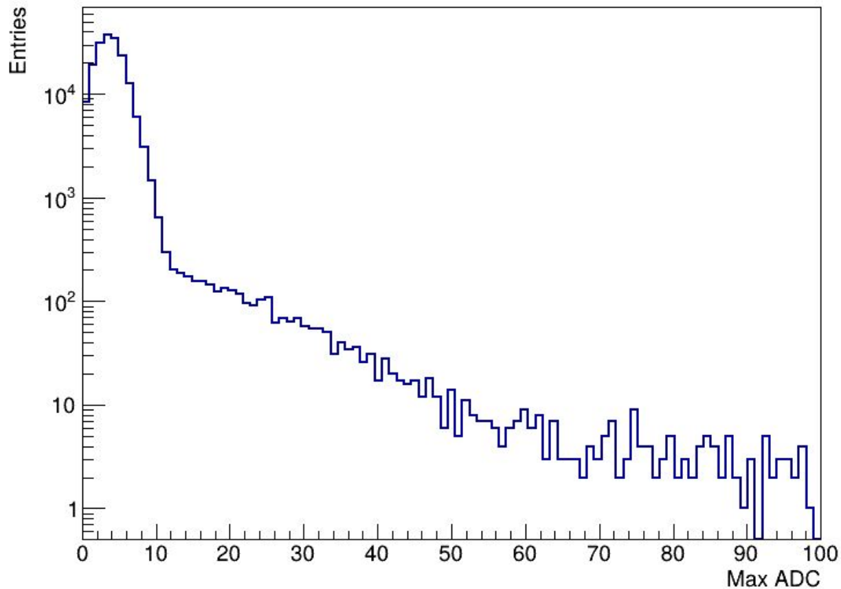
Max ADC distribution | Channel 156
