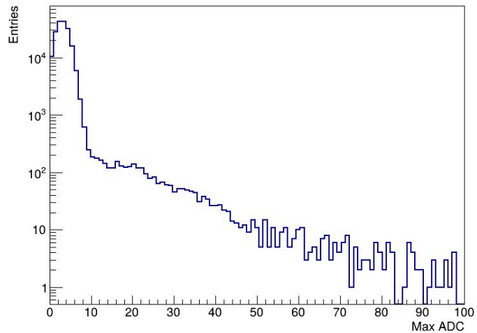
Max ADC distribution | Channel 156
