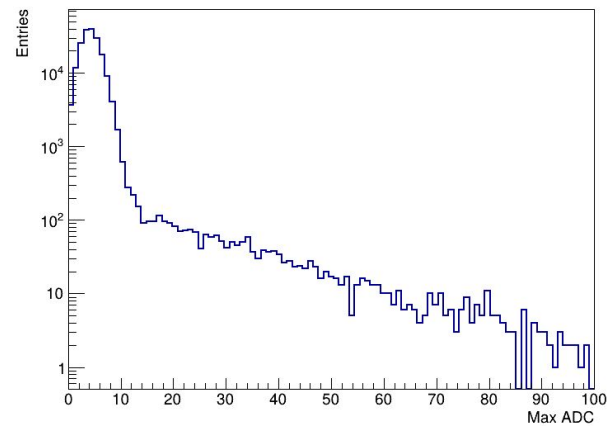
Max ADC distribution | Channel 93
