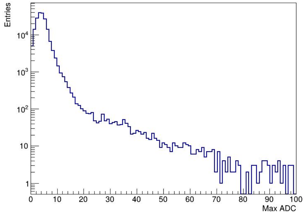
Max ADC distribution | Channel 93
