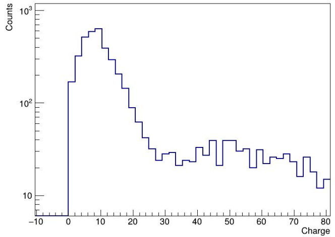
Charge Ch 79
