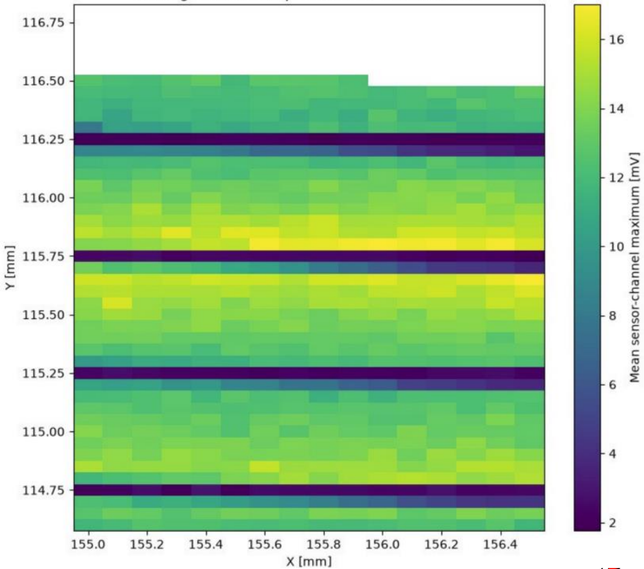
average: live XY amplitude at Z=157.286 mm
