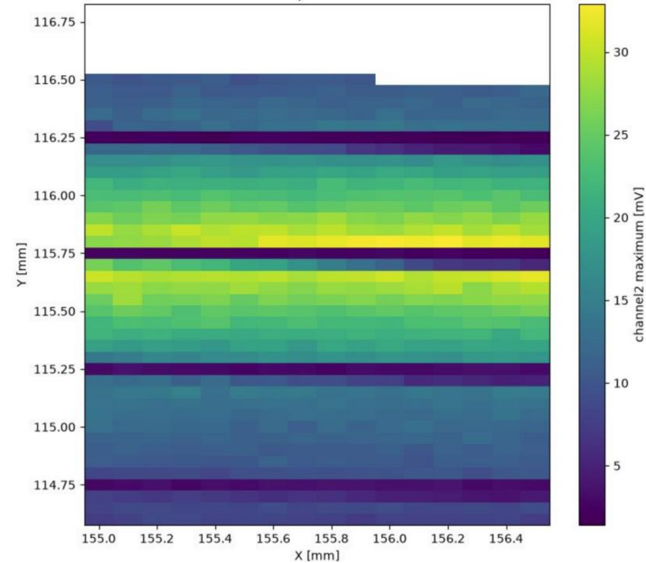
channel2: live XY amplitude at Z=157.286 mm
