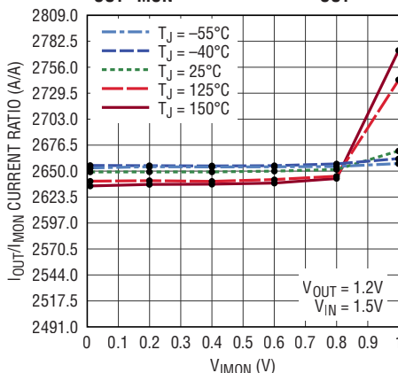
I_{OUT}/I_{MON} Current Ratio, I_{OUT} = 3A
