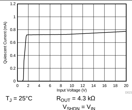
Figure 8. Quiescent Current vs Input Voltage
