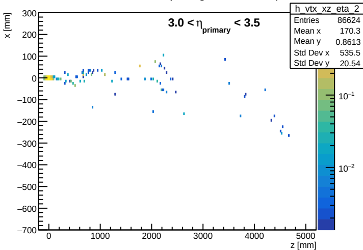
Emission Vertex of Depositing Particle, 3.0 < \eta < 3.5
