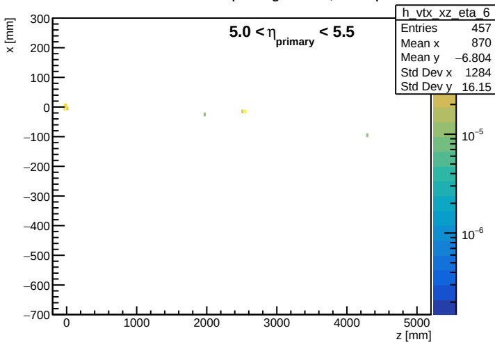
Emission Vertex of Depositing Particle, 5.0 < \eta < 5.5
