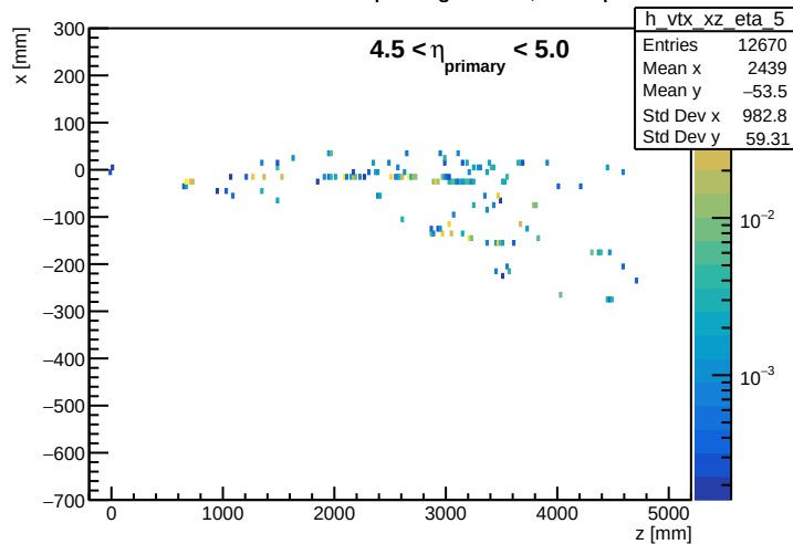
Emission Vertex of Depositing Particle, 4.5 < \eta < 5.0
