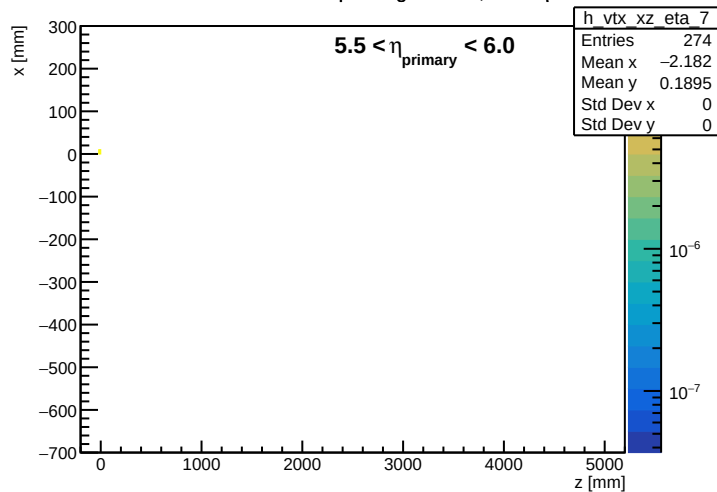
Emission Vertex of Depositing Particle, 5.5 < \eta < 6.0
