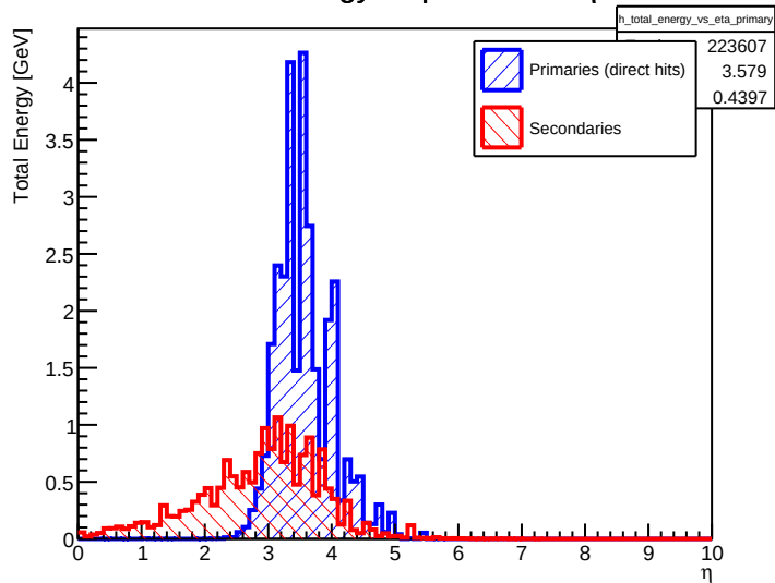
Total Energy Deposition vs \eta
