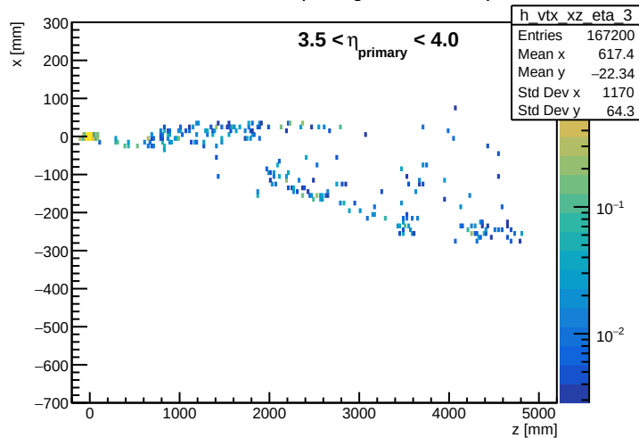
Emission Vertex of Depositing Particle, 3.5 < \eta < 4.0
