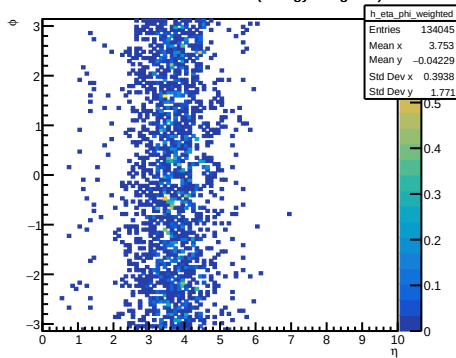
Generator Level Particles (Energy Weighted)
