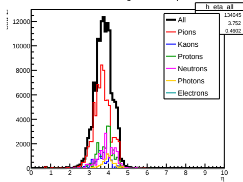
All Particles Contributing to HcalEndcapPInsert
