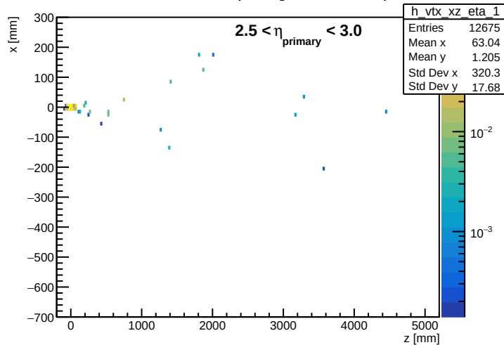
Emission Vertex of Depositing Particle, 2.5 < \eta < 3.0
