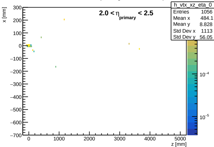
Emission Vertex of Depositing Particle, 2.0 < \eta < 2.5
