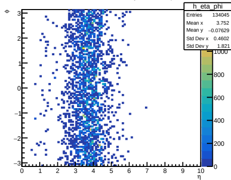
Generator Level Particles Contributing to HcalEndcapPInsert
