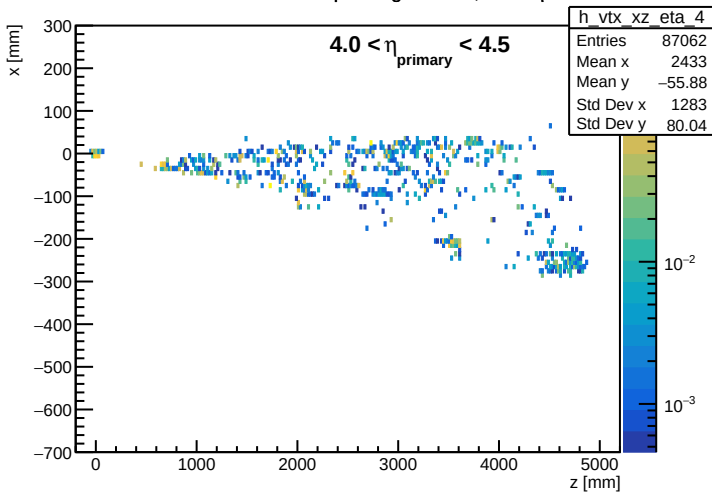
Emission Vertex of Depositing Particle, 4.0 < \eta < 4.5
