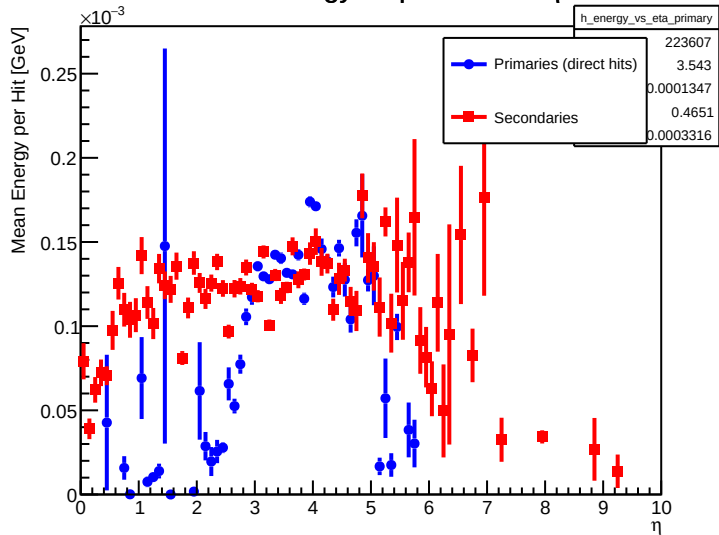
Mean Energy Deposition vs \eta
