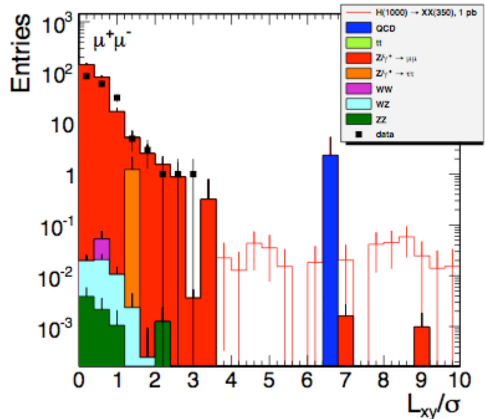
CMS Preliminary \sqrt{s}=7 TeV L=1.2 \text{ fb}^{-1}
