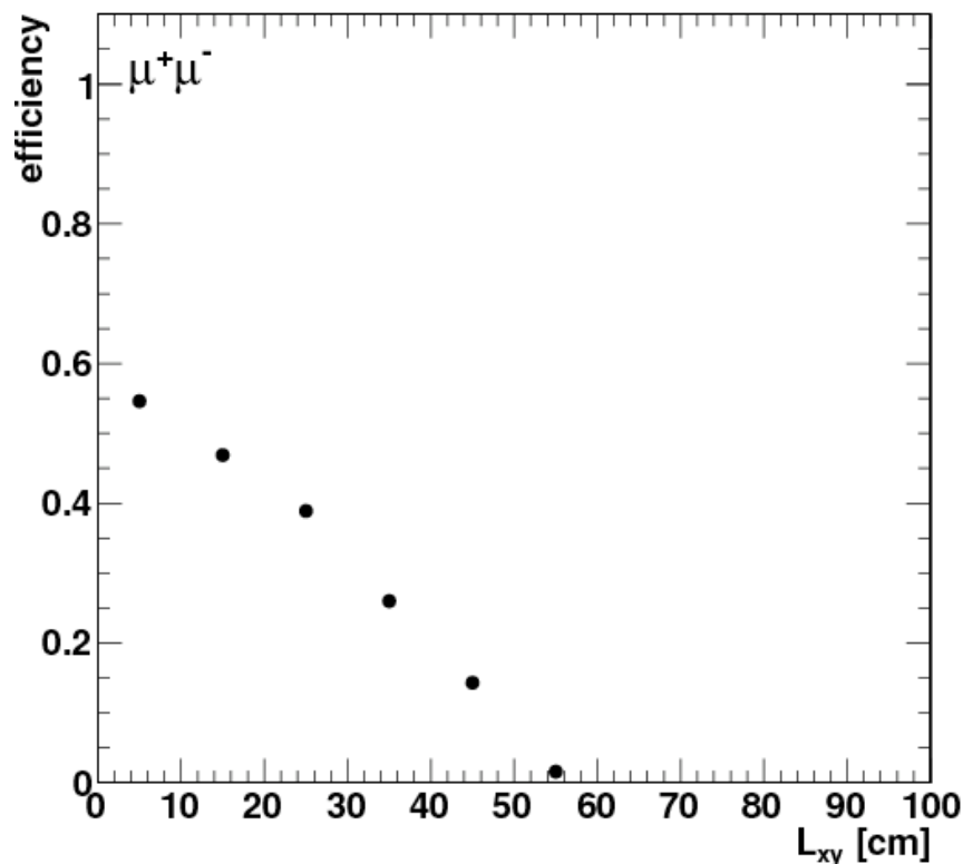
CMS Preliminary \sqrt{s}=7 TeV MC
