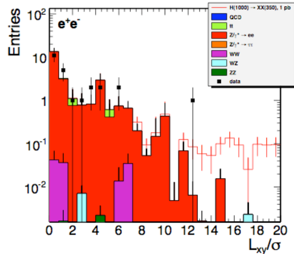
CMS Preliminary \sqrt{s}=7 TeV L=1.1 \text{ fb}^{-1}
