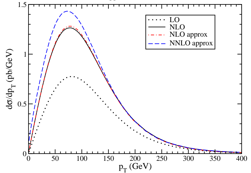
Top quark p_T distribution at LHC S^{1/2}=8 TeV \mu=m_t=173 GeV gg \rightarrow t\bar{t} channel
