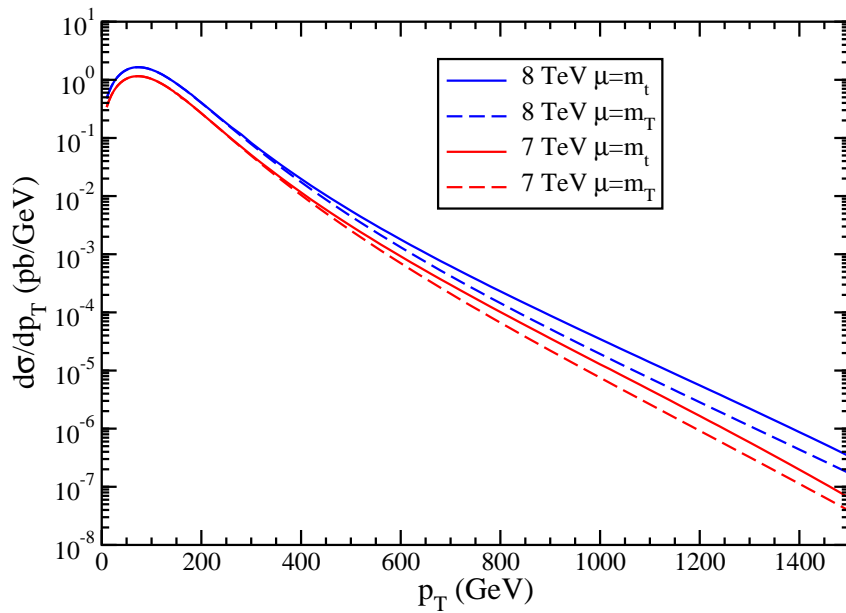
Top quark p_T distribution at LHC NNLO approx m_t=173 GeV
