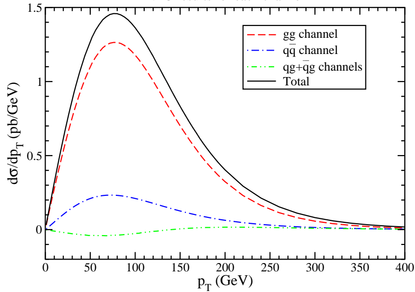
Top quark p_T distribution at LHC S^{1/2}=8 TeV \mu=m_t=173 GeV NLO results for each channel
