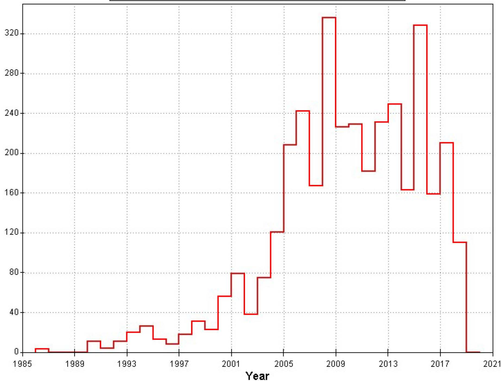
ENSDF nuclide age distribution, total=3577, mean=9.48
