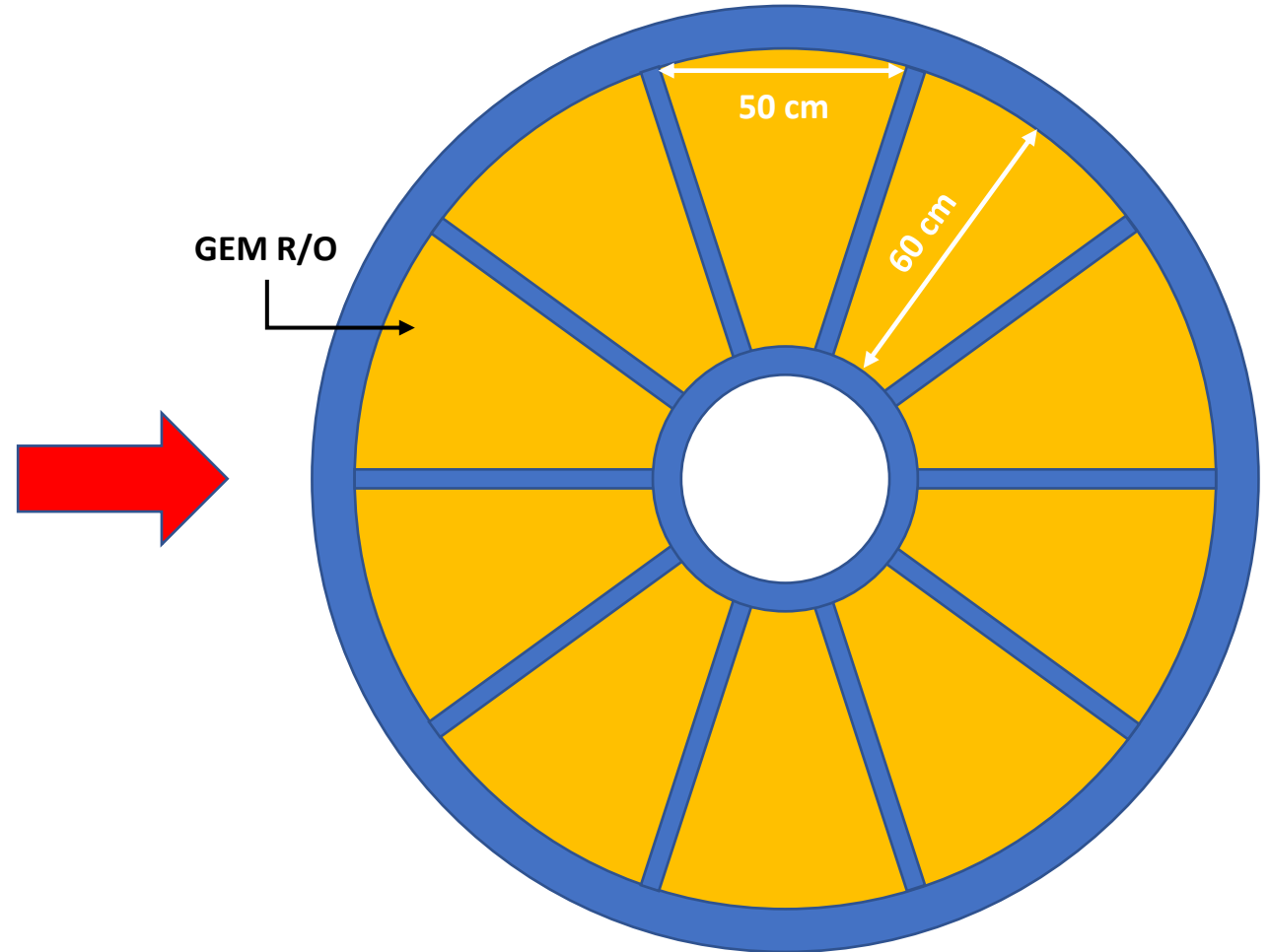
EIC TPC Wagon Wheel with 10 larger GEM readout modules
