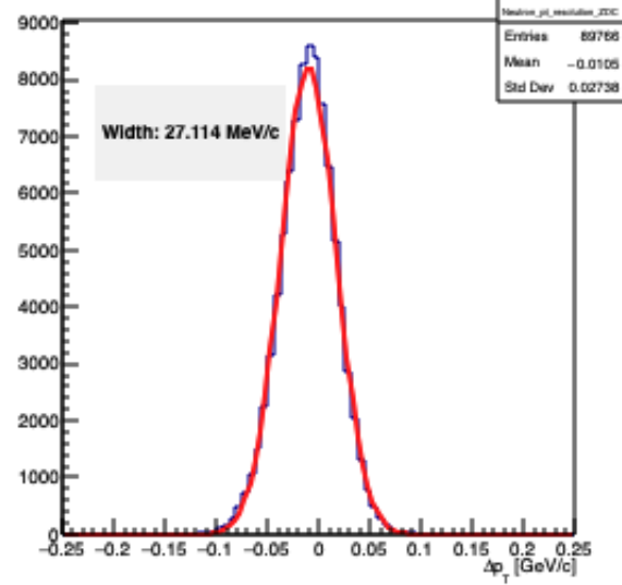
neutron_pt_resolution_ZDC
