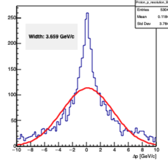
proton_p_resolution_B0
