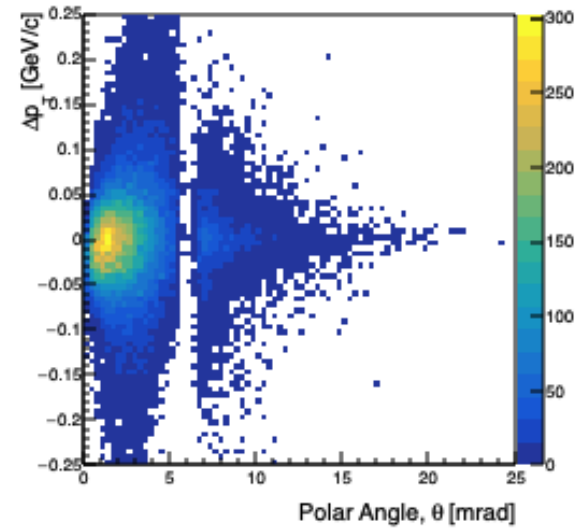
neutron_delta_pt_vs_theta
