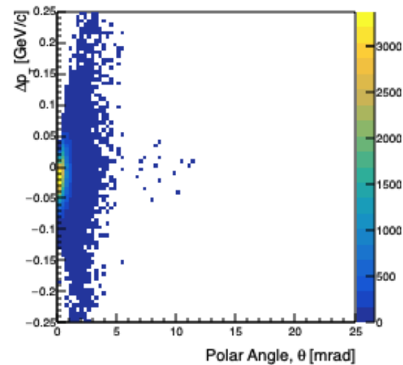
neutron_delta_pt_vs_theta
