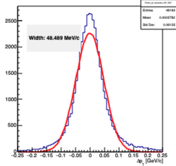
proton_pt_resolution_RP_EXT
