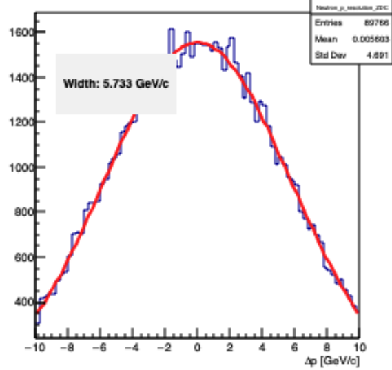
neutron_p_resolution_ZDC
