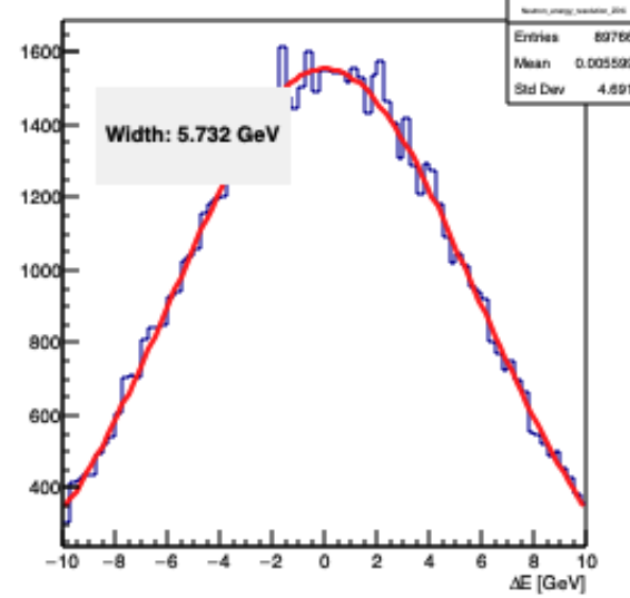
neutron_energy_resolution_ZDC
