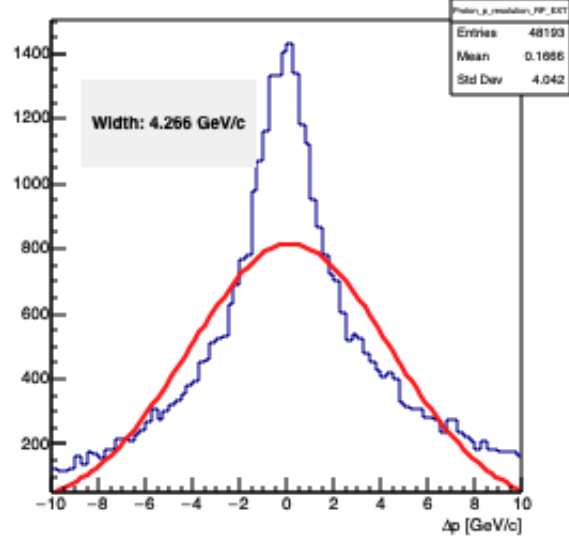
proton_p_resolution_RP_EXT
