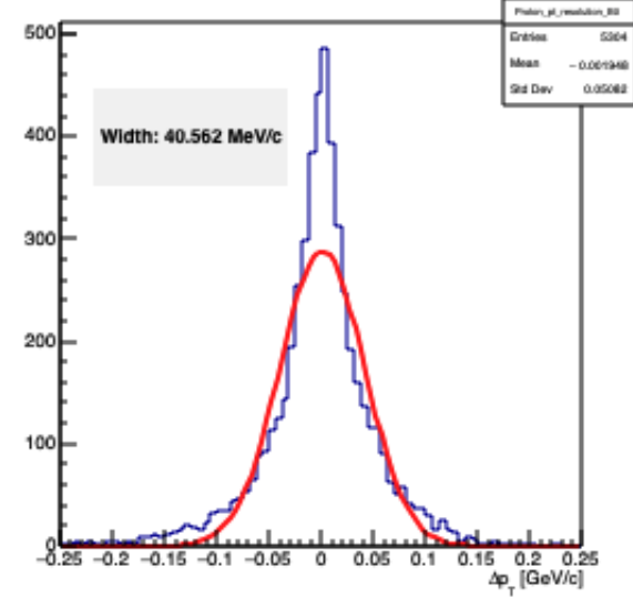
proton_pt_resolution_B0
