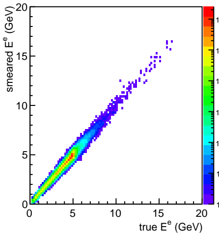
smear electron E
