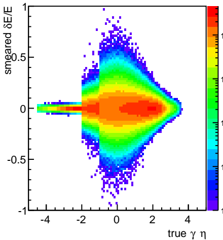
smear photon \delta E/E vs. \eta
