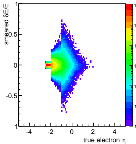
smear electron E
