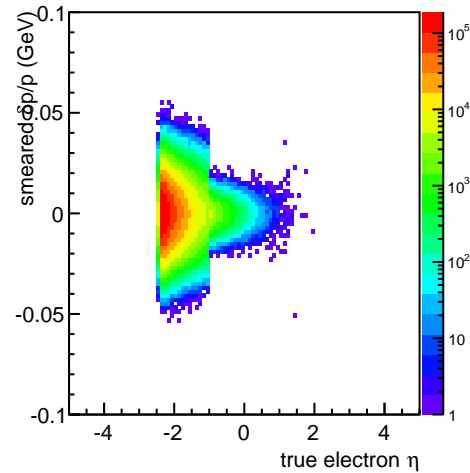
smear electron \delta p/p vs. \eta
