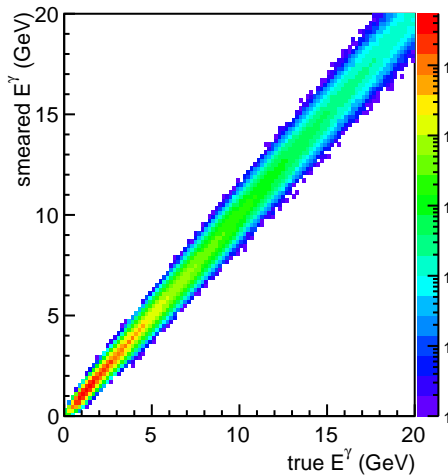
smear photon E
