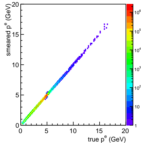
smear electron p
