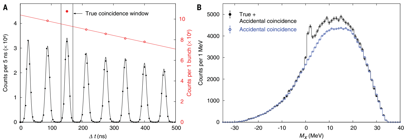
Fig. 2. Accidental-coincidence background distributions from the coincident timing spectrum and missing-mass spectrum for the ^{112}\text{Sn} target. (A) Coincident time spectrum of the protons and \alpha particles in the time window of the 500-ns coincidence gate. (B) Missing-mass spectrum (black: true and accidental-coincidence events; blue: only accidental-coincidence events).
