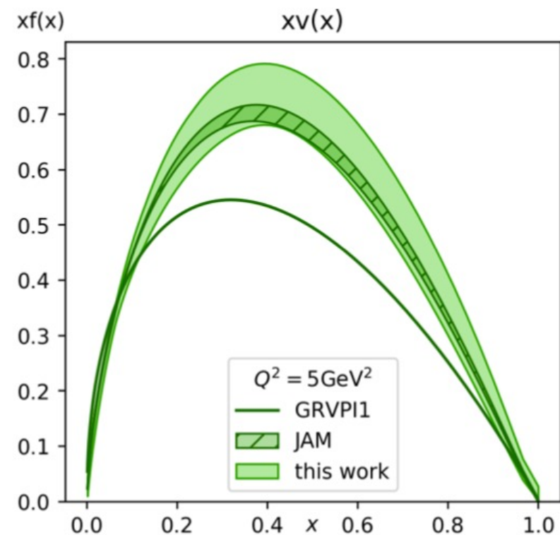
xFitter
