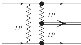
absorptive correction
